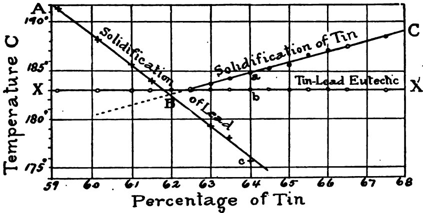
Fig. 25. Freezing-point Curve of Lead-tin Alloys. Roberts-Austen, Proc. Royal Soc. , LXIII, p. 452.
